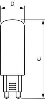
CorePro LEDcapsule ND 4.8-60W G9 827
