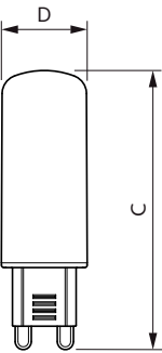
G9 230V 5W-55W 600lm 36D 3000K GU9 ND
