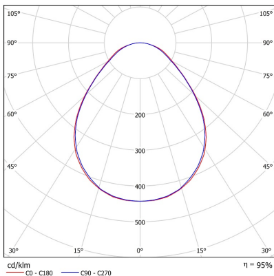
COMPACT LED 50W PRM 600×600 3000K
